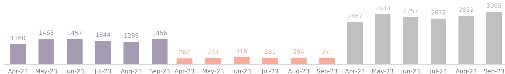
Finance, Statistics
